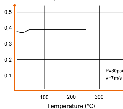
Friction coefficient \mu
