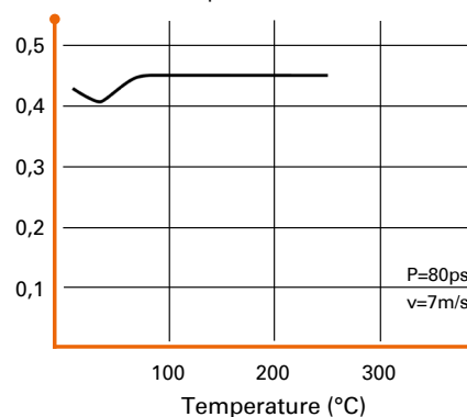
Friction coefficient \mu
