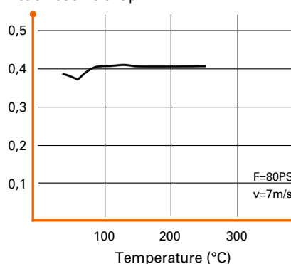
Friction coefficient \mu
